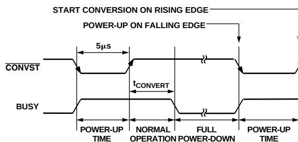
Figure 24. Power-Up Timing When Using \overline{\text{CONVST}} Pin
