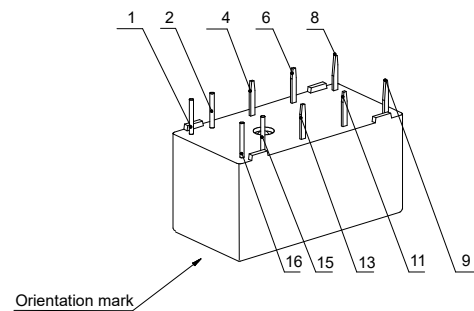
2 coils latching
