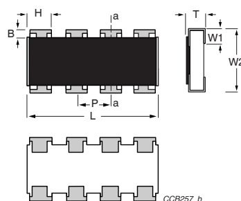
Fig. 3 YC324 series chip resistors dimension
