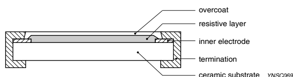
Fig. 2 Chip resistor outlines
