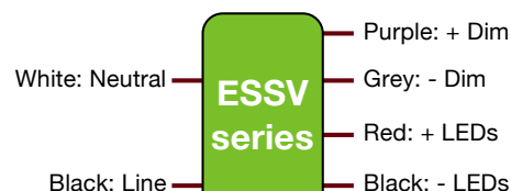
Wiring Diagram
