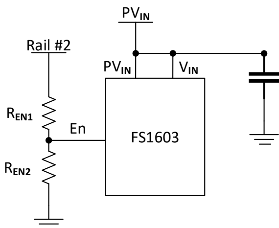
Figure 10 En pin used to monitor other rails for sequencing purposes
