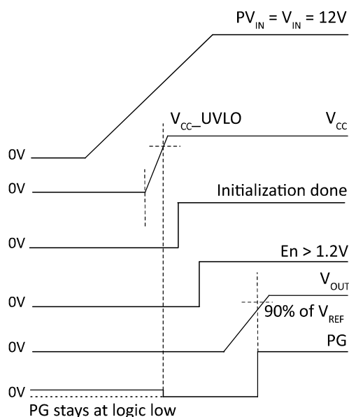
Figure 10 En pin used to monitor other rails for sequencing purposes
