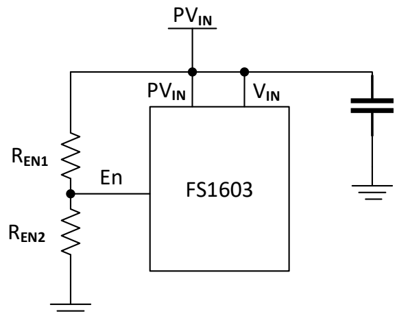
Figure 6 Single supply configuration: internal LDO regulator, adjustable PV_{IN\_UVLO}
