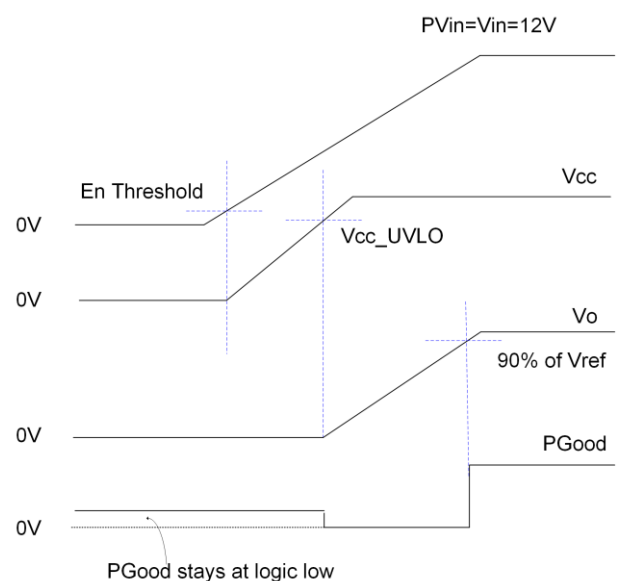
Figure 9 Start-up: PV_{IN} , V_{IN} tied together, En connected to resistor divider from PV_{IN} , PG pin pulled up to an external supply
