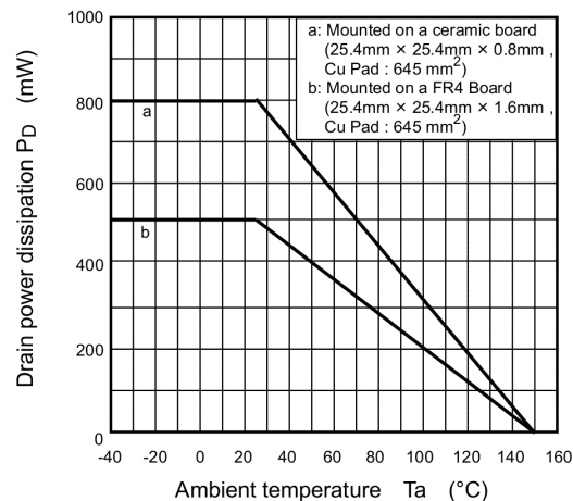
Fig. 7.12 P_D - T_a
