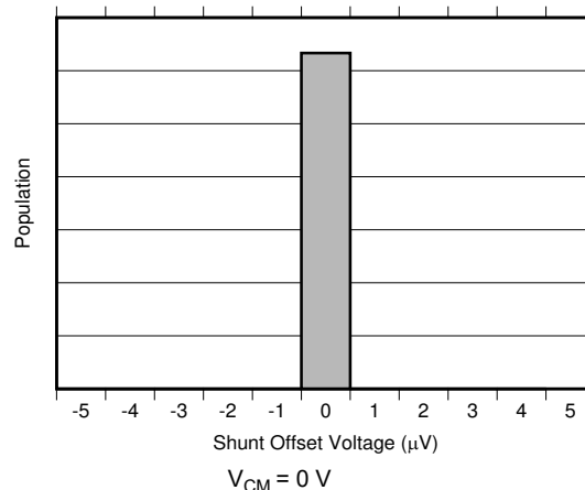
Figure 6-3. Shunt Input Offset Voltage Production Distribution
