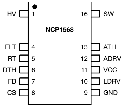
Figure 2. Pinout
