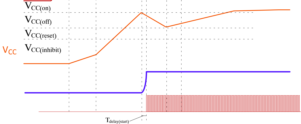
Figure 6. Normal Startup Timing Diagram and Delays
