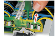
CAGE CLAMP® connection Removing a solid conductor.
