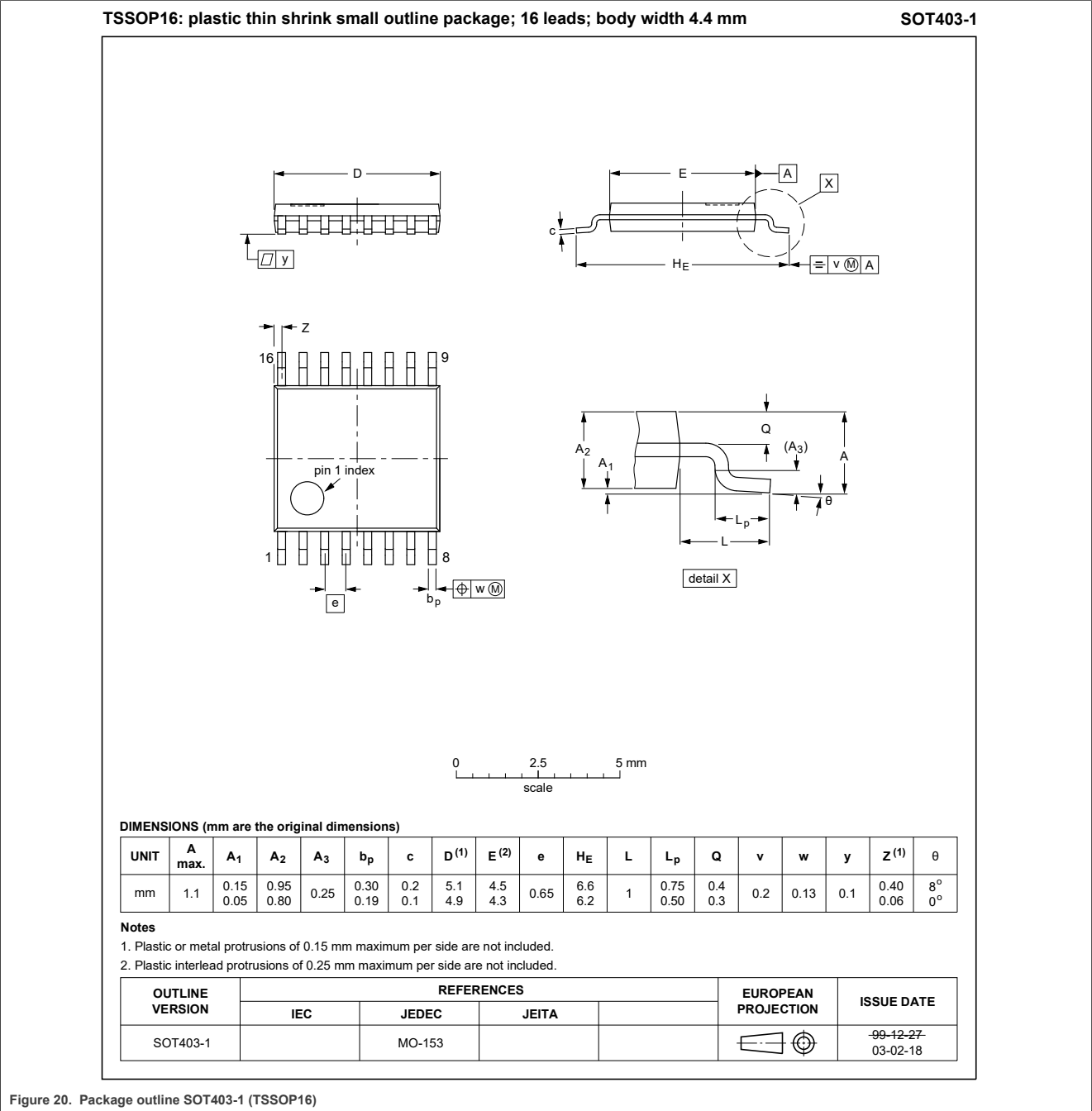
Figure 20. Package outline SOT403-1 (TSSOP16)
