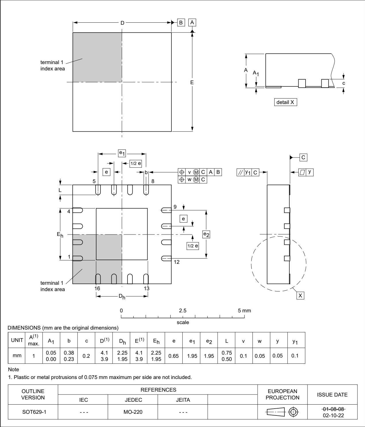
Figure 21. Package outline SOT629-1 (HVQFN16)
