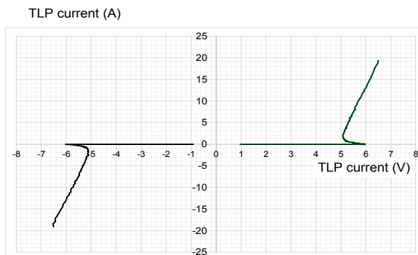
Figure 6. TLP characteristic
