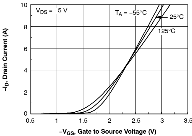
Figure 5. Transfer Characteristics
