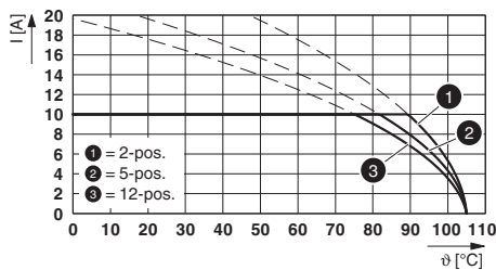
Type: FKCVW 2,5/...-ST with MDSTBW 2,5/...-G
