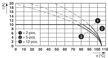
Type: FKCVR 2,5/...-ST with MDSTBW 2,5/...-G
