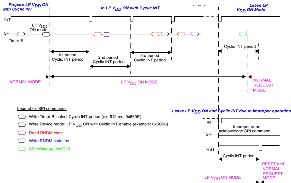
Figure 29. Cyclic Interrupt Operation
