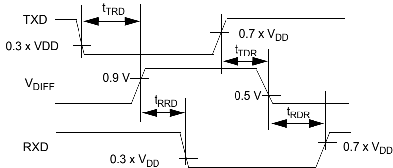
Figure 18. CAN Signal Propagation Delays TXD to CAN and CAN to RXD
