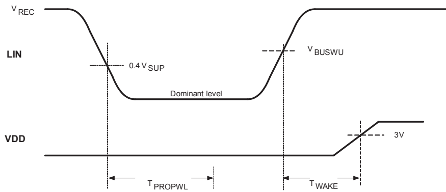
Figure 22. LIN Wake-up LP V_{DD} OFF Mode Timing
