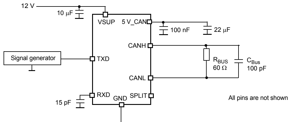
Figure 19. Test Circuit for CAN Timing Characteristics
