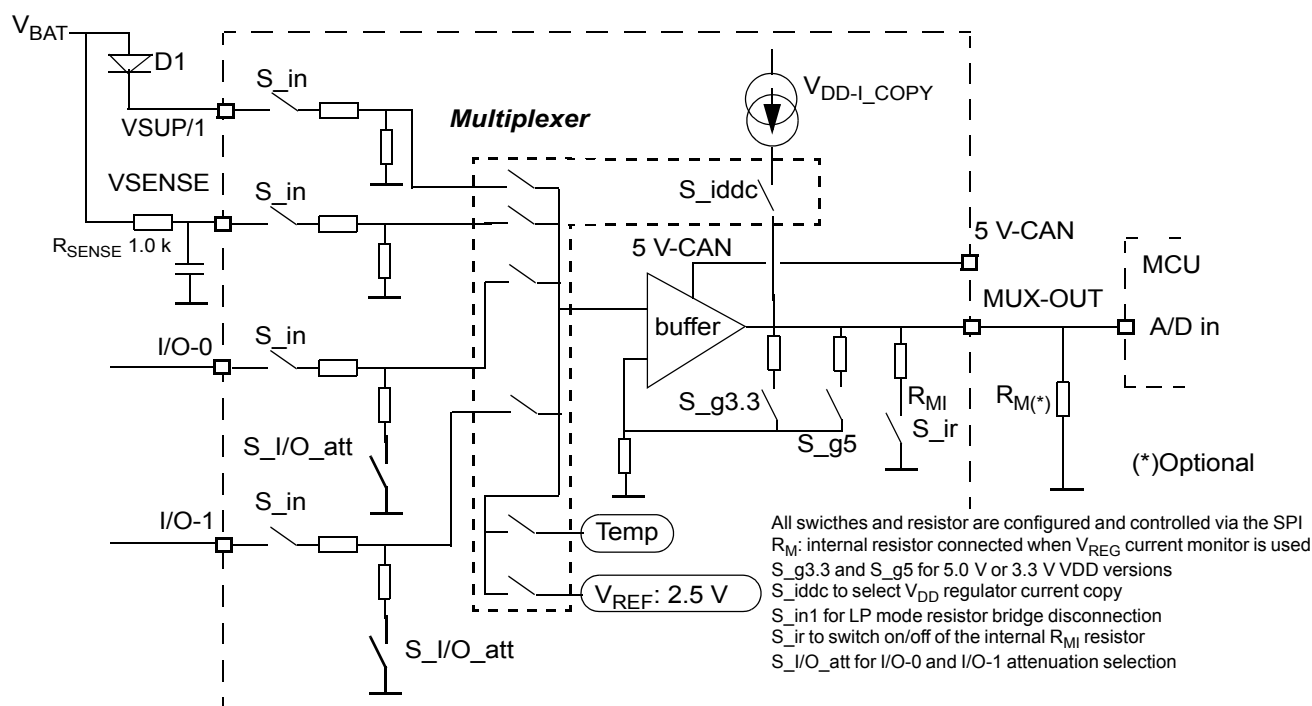
Figure 24. Analog Multiplexer Block Diagram
