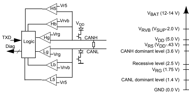
Figure 40. CAN Bus Simplified Structure Truth Table for Failure Detection
