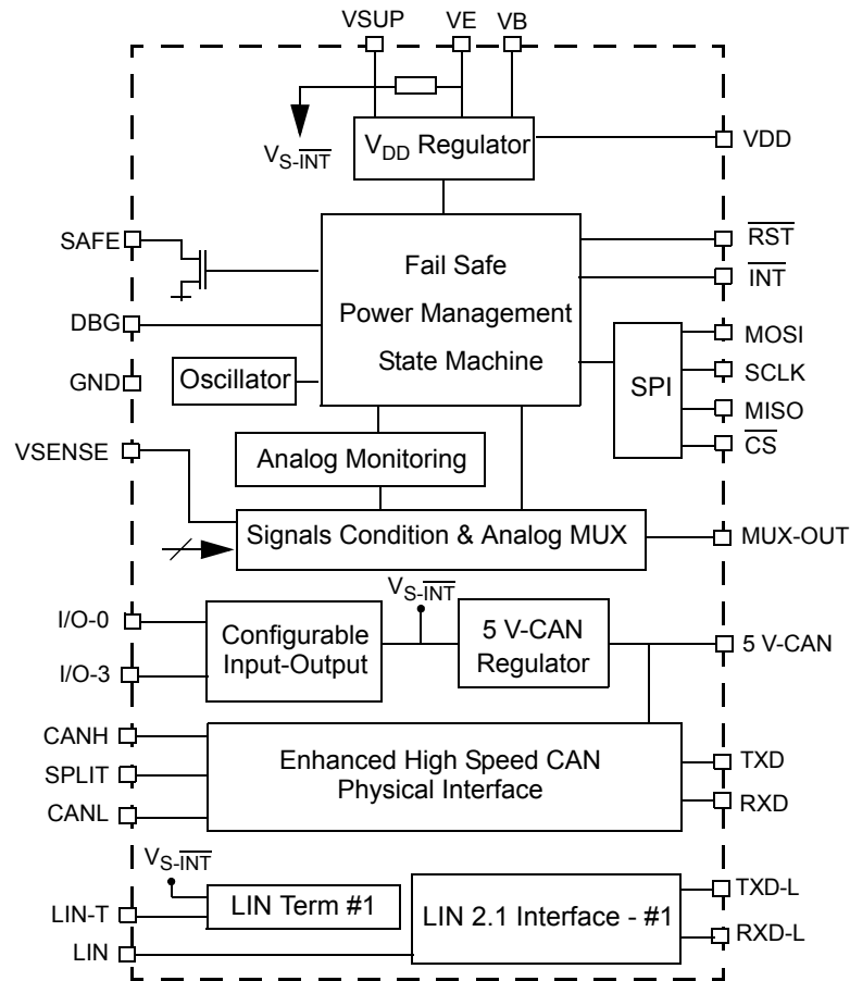
Figure 12. 33903S Internal Block Diagram
