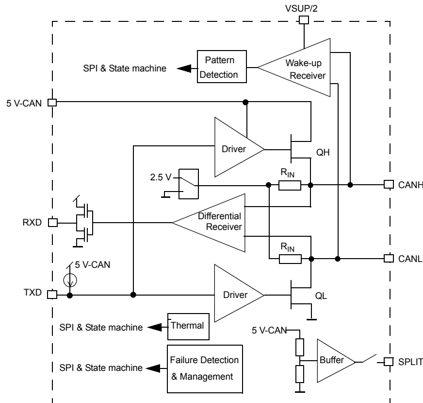
Figure 35. CAN Interface Block Diagram
