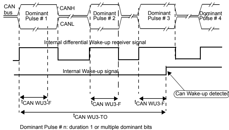
Figure 38. Pattern Wake-up - Multiple Dominant Detection
