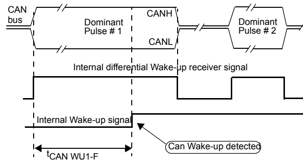
Figure 37. Single Dominant Pulse Wake-up
