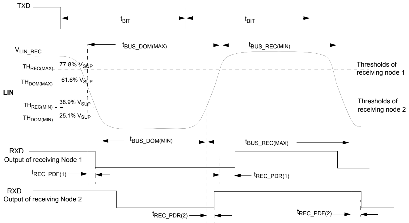
Figure 21. LIN Timing Measurements for Slow Slew Rate
