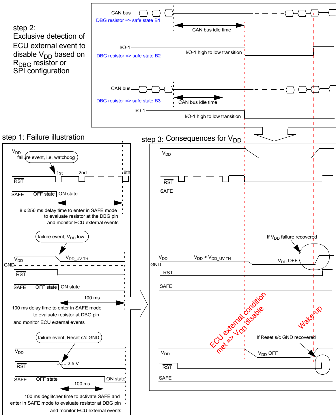
Figure 34. SAFE Modes B1, B2, or B3 Behavior Illustration
