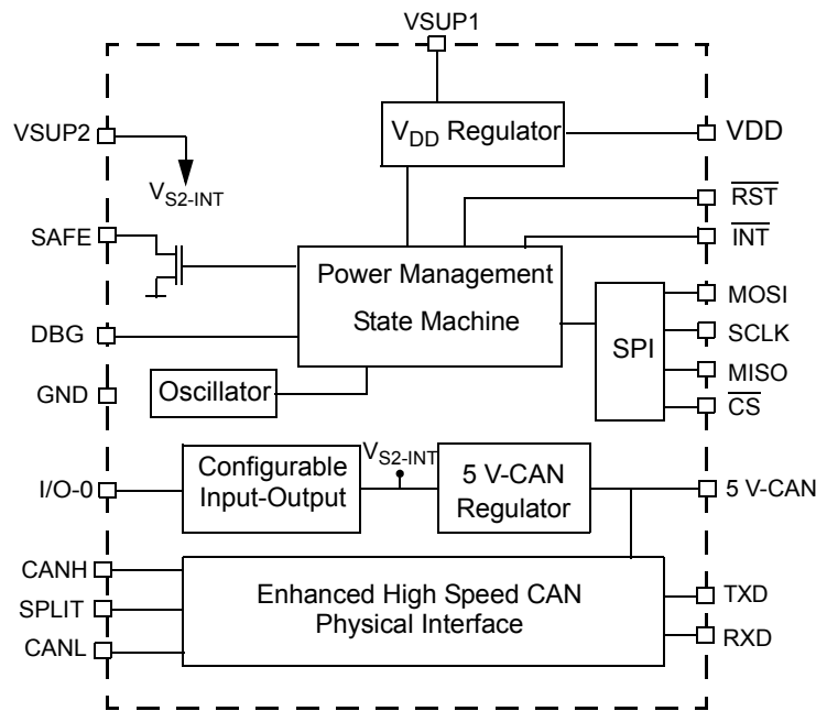
Figure 10. 33903 Internal Block Diagram
