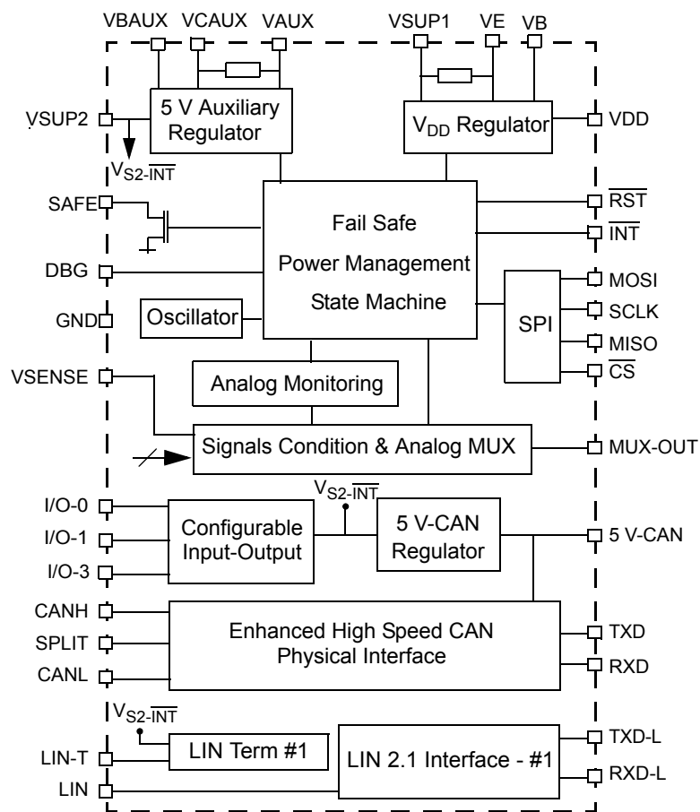
Figure 8. 33905S Internal Block Diagram
