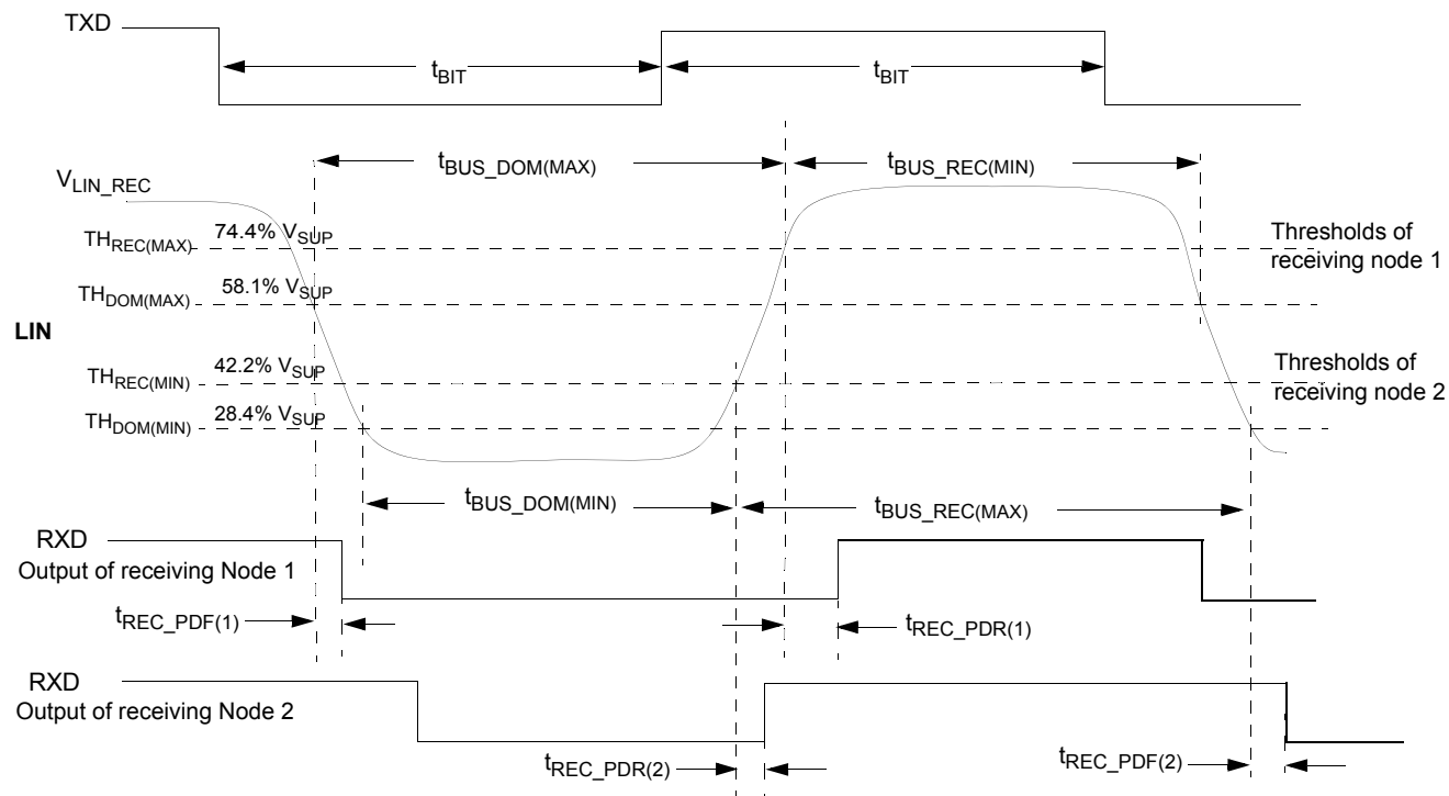
Figure 20. LIN Timing Measurements for Normal Slew Rate
