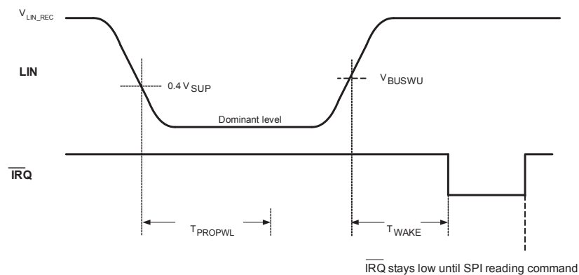
Figure 23. LIN Wake-up LP V_{DD} ON Mode Timing
