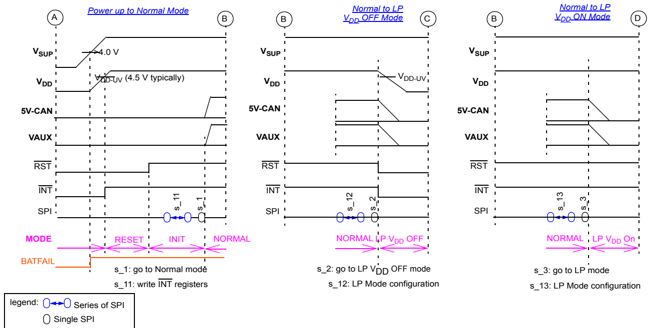
Figure 26. Power Up Normal and LP Modes
