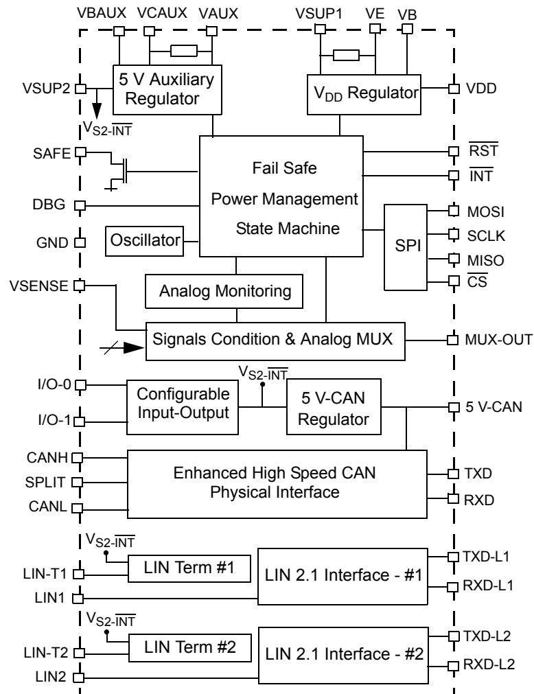
Figure 7. 33905D Internal Block Diagram
