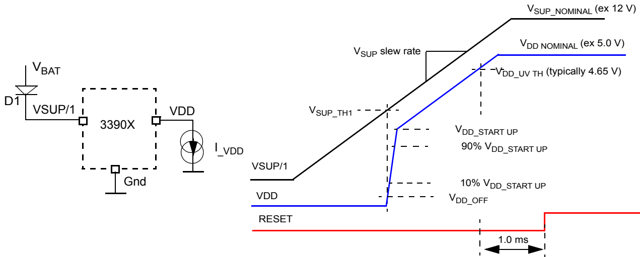
Figure 30. V_{DD} Start-up Versus V_{SUP/1} Tramp
