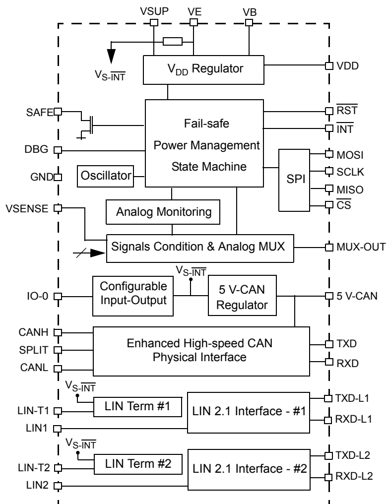
Figure 11. 33903D Internal Block Diagram
