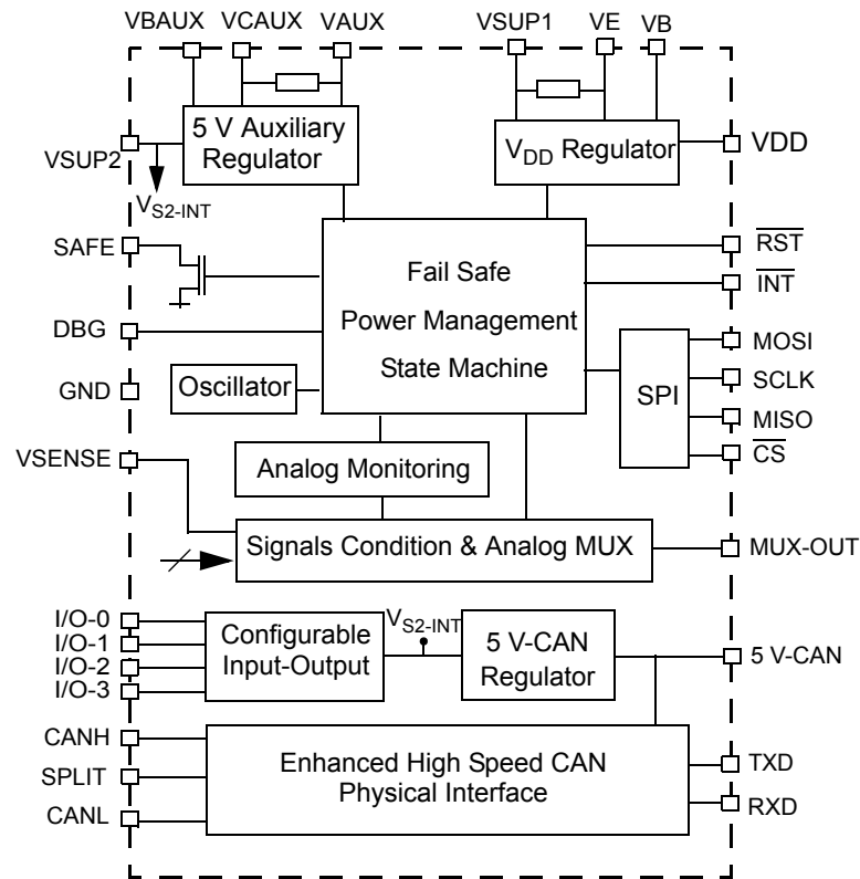
Figure 9. 33904 Internal Block Diagram
