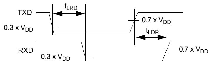
Figure 17. CAN Signal Propagation Loop Delay TXD to RXD
