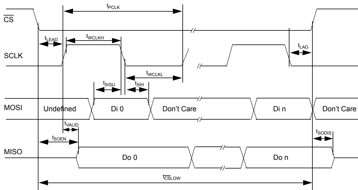
Figure 16. SPI Timings
