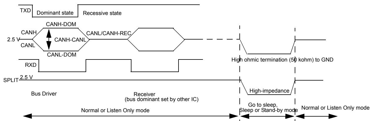
Figure 36. Bus Signal in TXD/RXD and LP Mode
