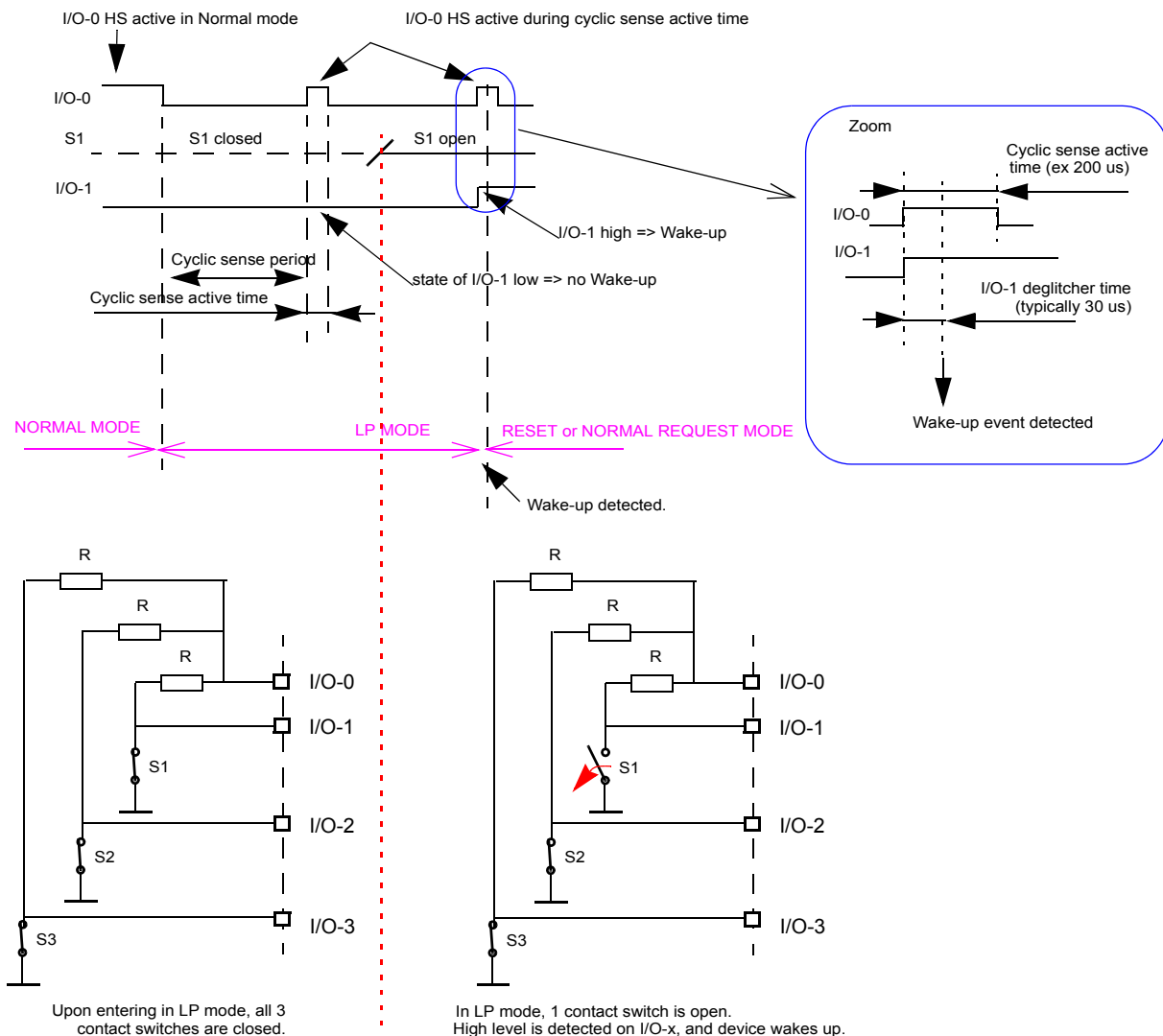
Figure 28. Cyclic Sense Operation - Switch to GND, Wake-up by Open Switch
