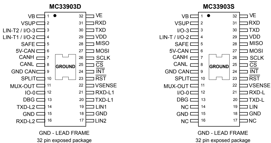
Figure 14. 33905D, MC33905S, MC33904 and MC33903 Pin Connections
