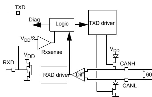
Figure 41. RXD Path Simplified Schematic, RXD Short to V_{DD} Detection
