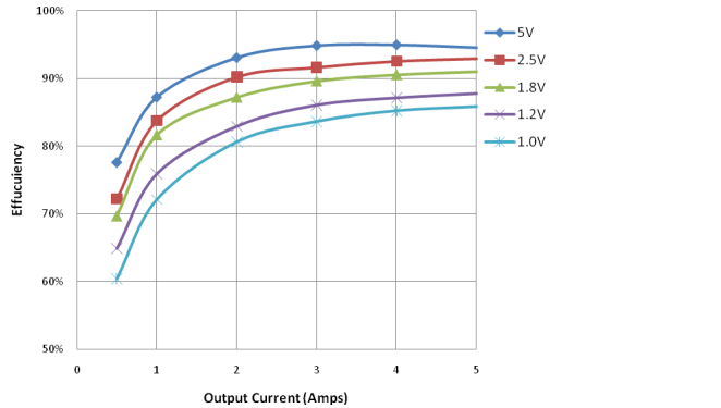
Fig. 4: 12Vin Efficiency: Single Channel 300kHz - Channels not in use are disabled FET: Si4944; Inductor: 744314xxx 7x7x5mm
