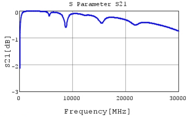
GJM0335C1E200FB01 S21 DCOV, 25degC
