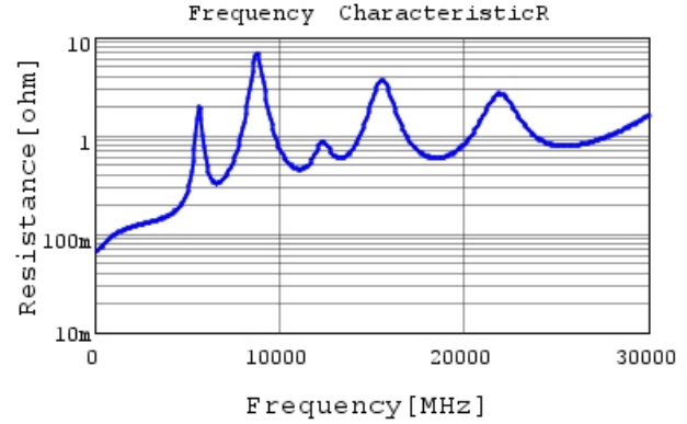
GJM0335C1E200FB01 R DCOV, 25degC
