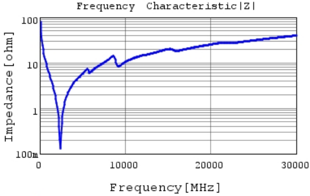
GJM0335C1E200FB01 |Z| DCOV, 25degC
