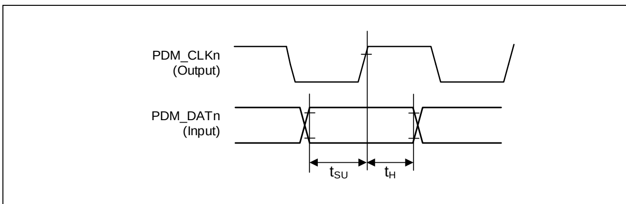
Figure 3.68 Receive Timing (Synchronized with the Rise of PDMn_CLK)
