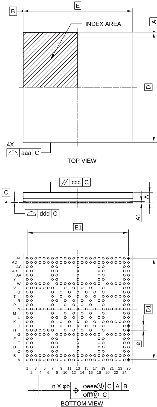
Figure 4.2 Package Dimensions (361Pin BGA)
