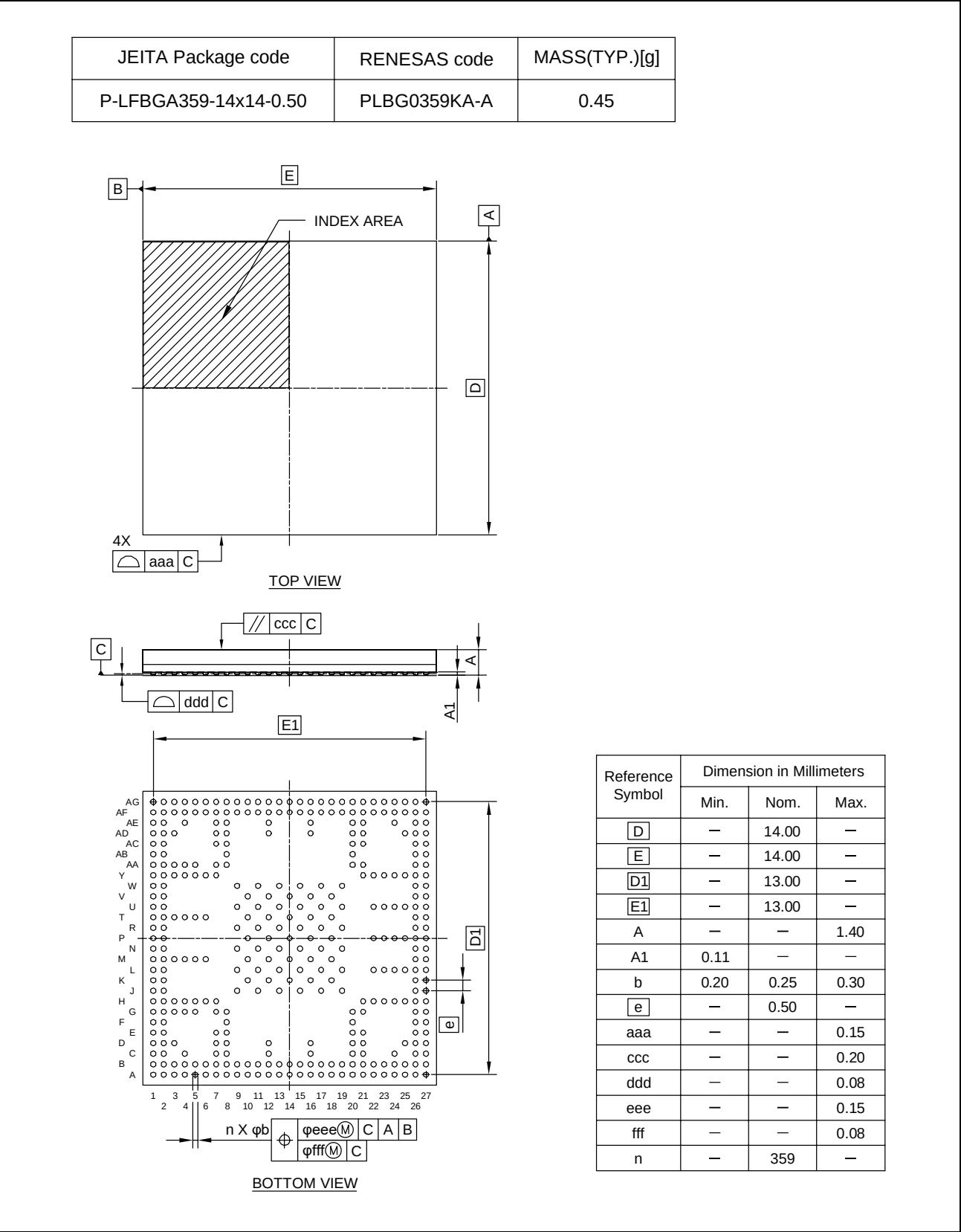
Figure 4.1 Package Dimensions (359Pin BGA)
