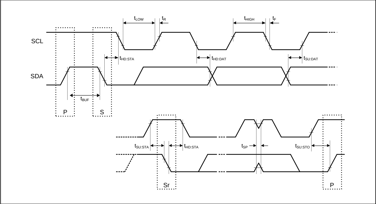
Figure 3.44 Input/Output Timing
