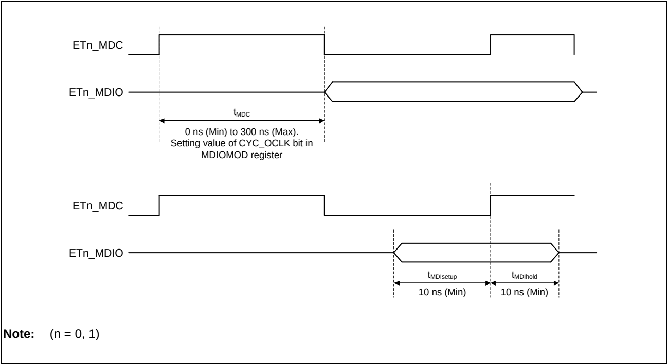
Figure 3.22 Management Interface
