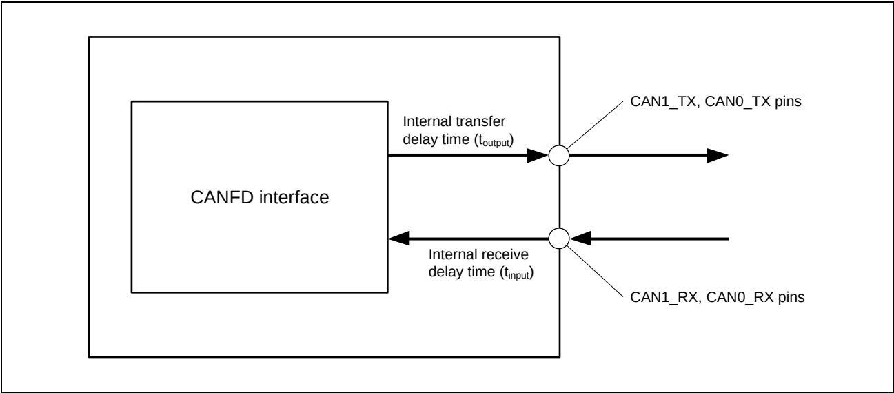
Figure 3.37 CAN-FD Interface Condition
