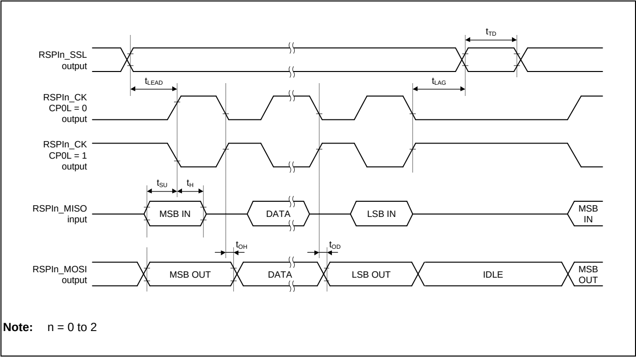
Figure 3.61 Transmission and Reception Timing (Master, CPHA = 0)
