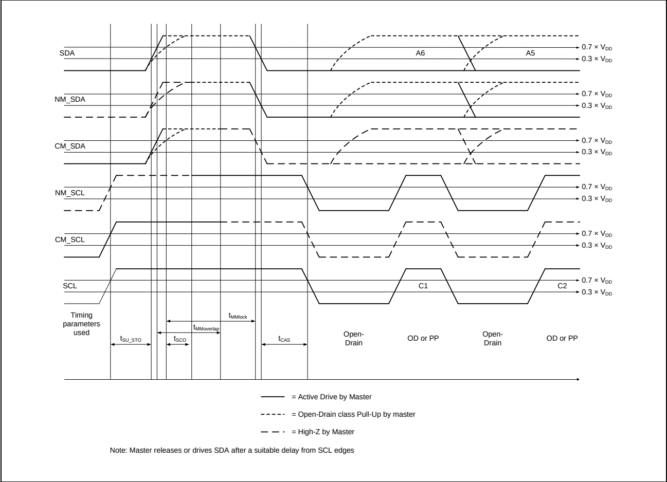
Figure 3.54 I3C Timing
