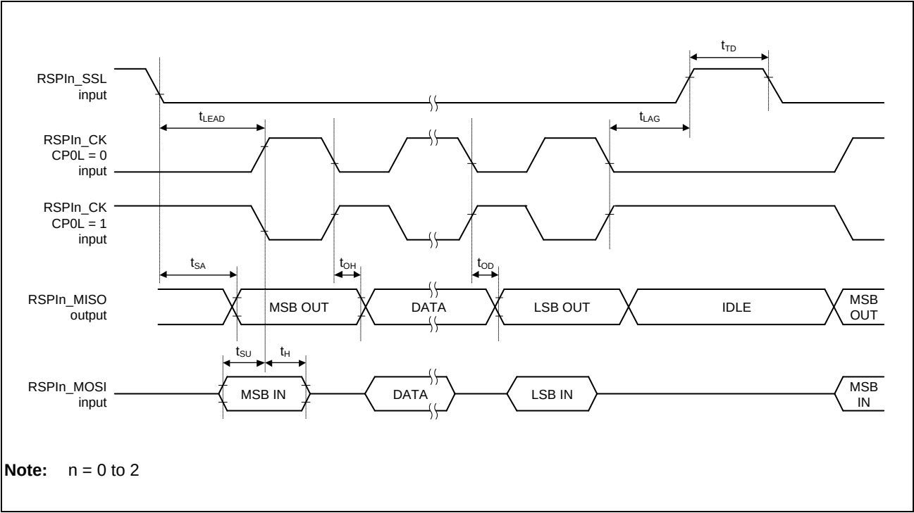
Figure 3.63 Transmission and Reception Timing (Slave, CPHA = 0)
