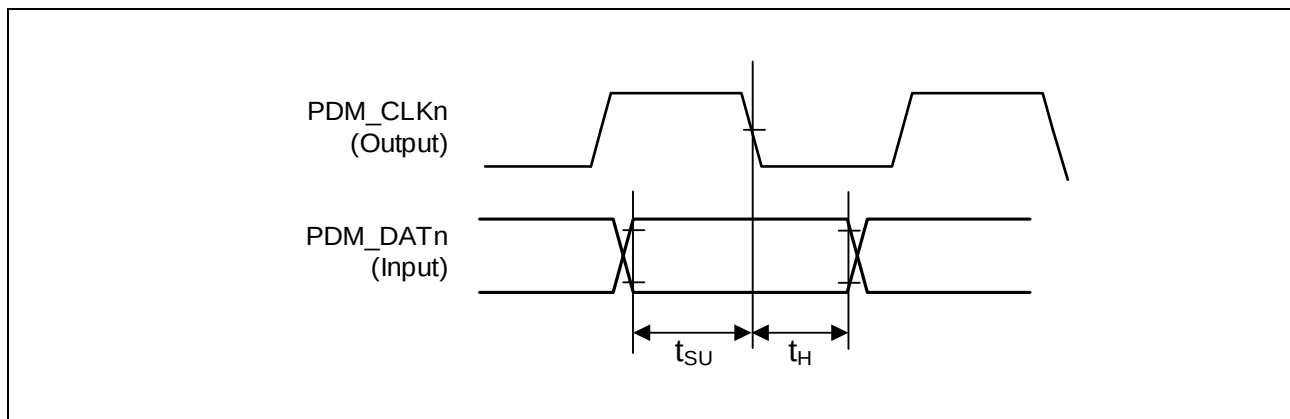
Figure 3.69 Receive Timing (Synchronized with the Fall of PDMn_CLK)
