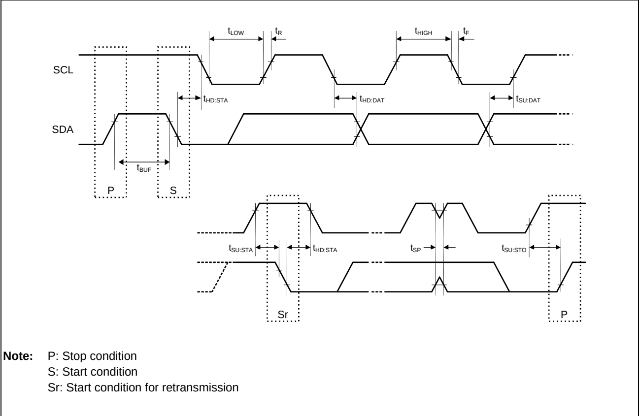
Figure 3.43 Input/Output Timing
