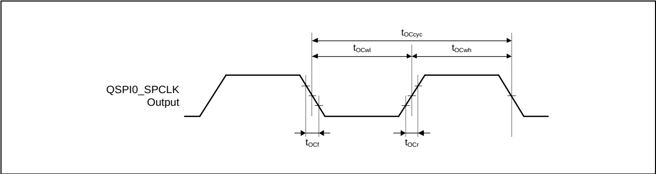
Figure 3.70 Clock Timing
