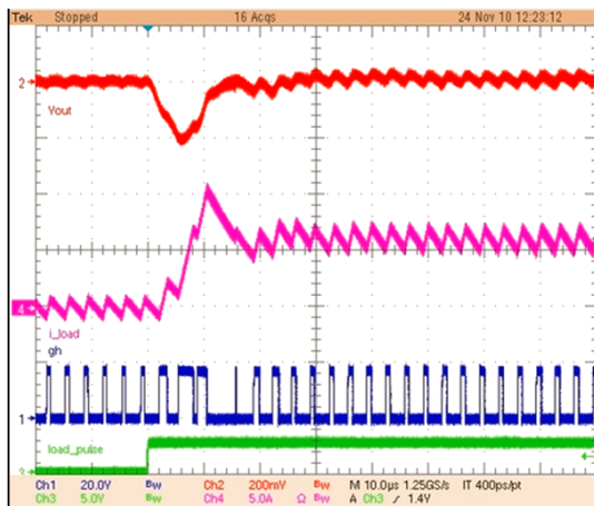
Figure 3: 0-6A Transient 300kHz PWM only
