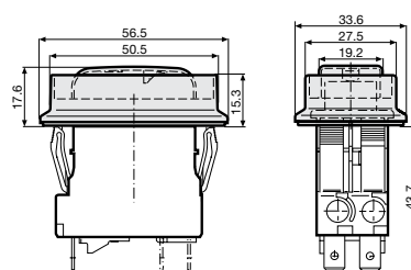
AZM11 / Partially raised collar with cover, narrow, IP54 AZM12 / Partially raised collar without cover, narrow, IP40
