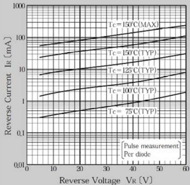
Reverse Current
