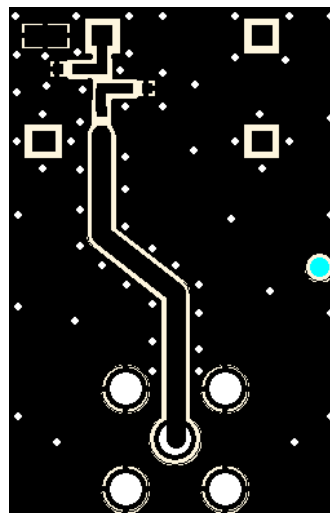
PCB Layout (from evaluation board)
