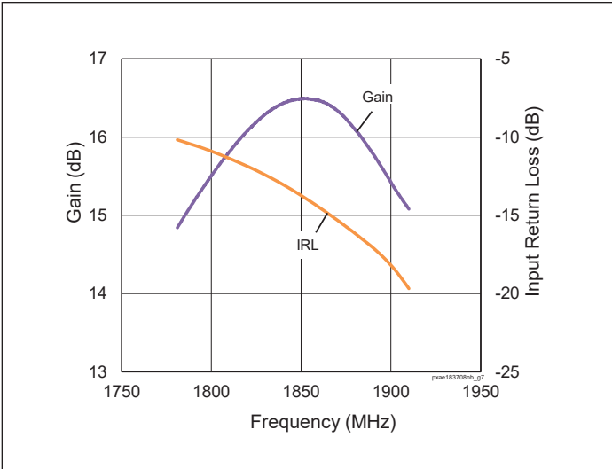
Figure 5. Small Signal CW Gain & Input Return Loss V_{DD} = 28\text{ V} , I_{DQ} = 800\text{ mA}
