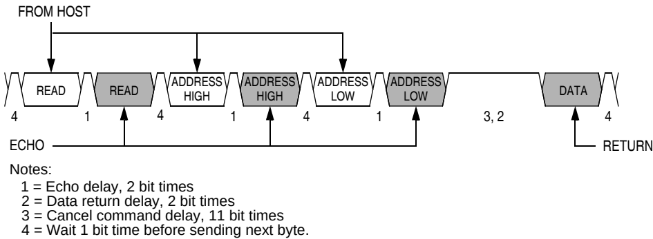
Figure 10-5. Read Transaction
