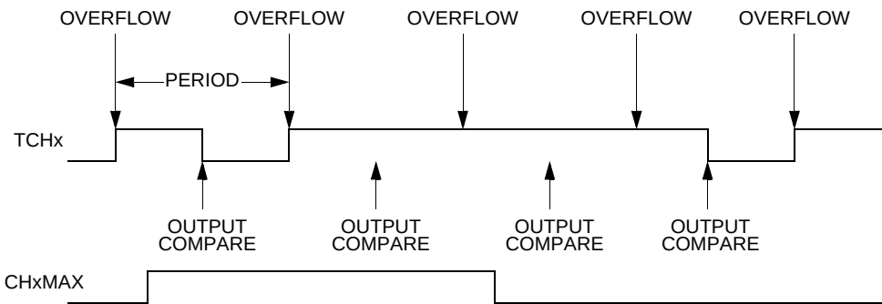
Figure 11-11. CHxMAX Latency
