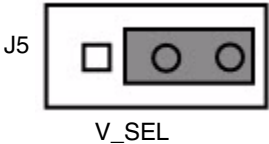
Figure 2-8. Jumper Placement for 3.3 V
