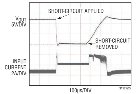
Short-Circuit Response
