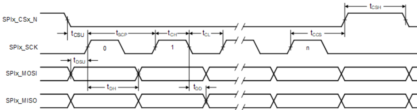
Figure 3 SPI Slave Timing Diagram
