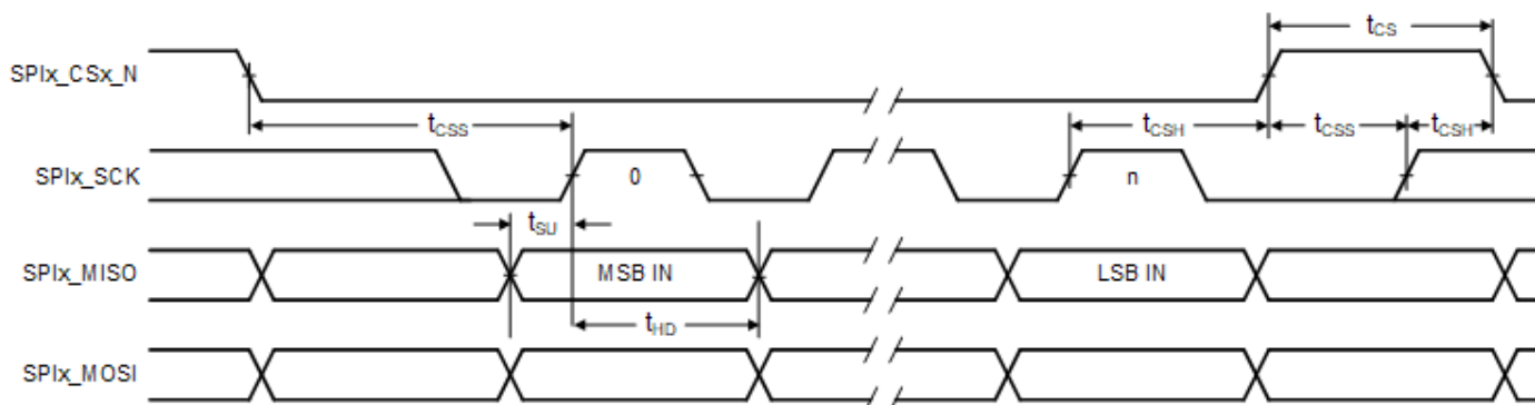
Figure 2 SPI Master Timing Diagram
