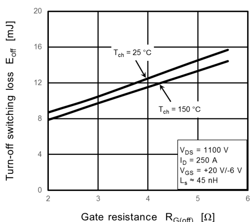
Fig. 8.11 E_{off} - R_{G(off)}
