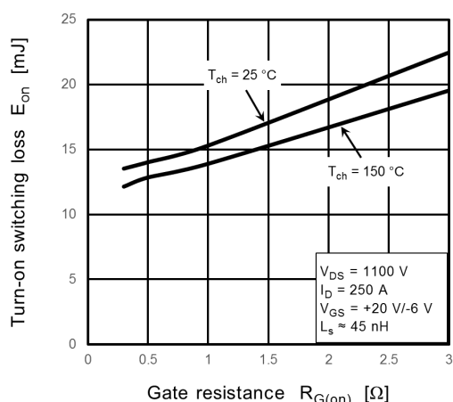
Fig. 8.10 E_{on} - R_{G(on)}
