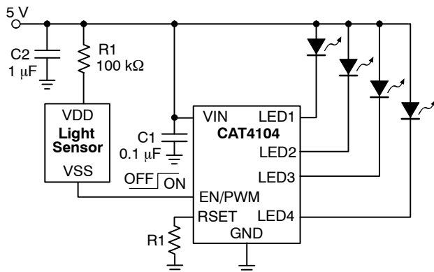
Figure 21. Daylight Detection
