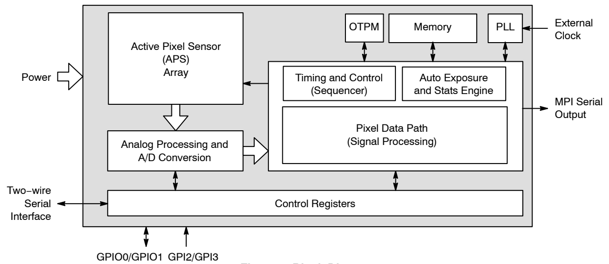
Figure 1. Block Diagram
