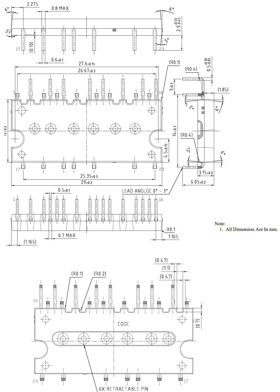
Figure 16 IM241-S6T2x (DIP 29x12)
