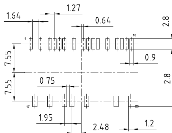
Figure 18 IM241-S61x (SOP 29x12)
