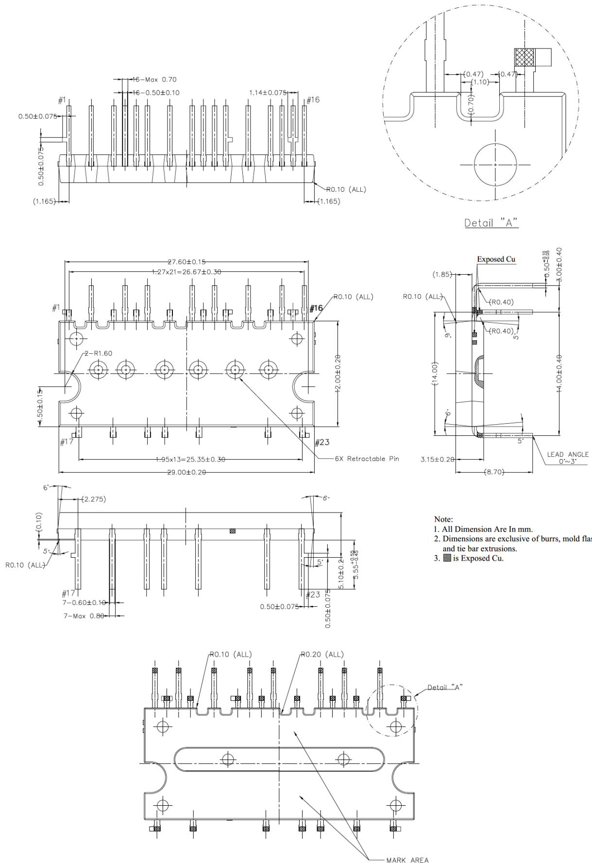
Figure 17 IM241-S6T2x2 (DIP 29x12)
