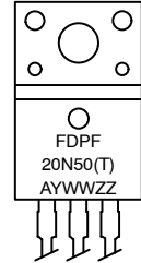
TO-220 Fullpack, 3-Lead / TO-220F-3SG CASE 221AT
