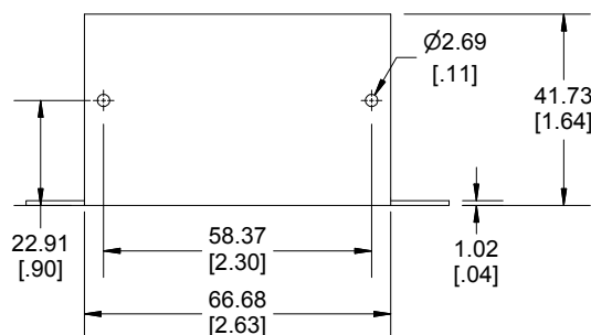
Side View of Flanged Bottom
