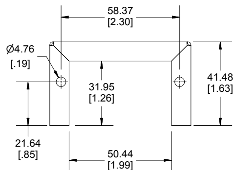
Side View of Cover
