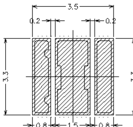
Soldering patterns
