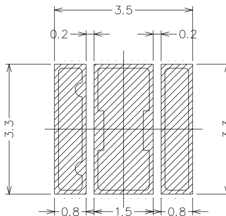
Soldering patterns
