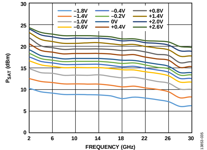
Figure 36. P_{SAT} vs. Frequency at Various V_{GG2} Voltages
