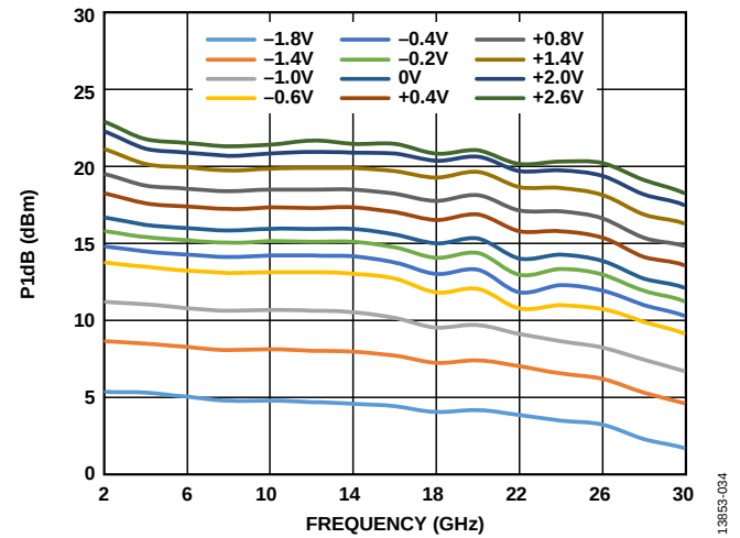
Figure 35. P1dB vs. Frequency at Various V_{GG2} Voltages
