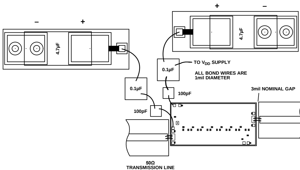
Figure 40. Assembly Diagram
