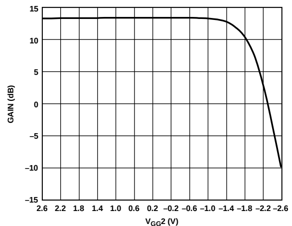
Figure 31. Gain vs. V_{GG2}
