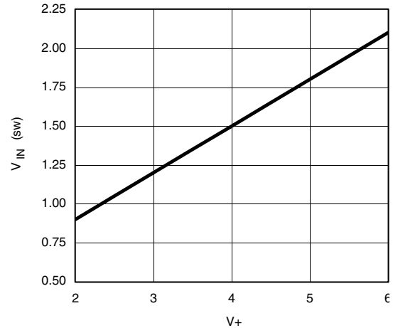
Input Switching Point vs. Power Supply Voltage
