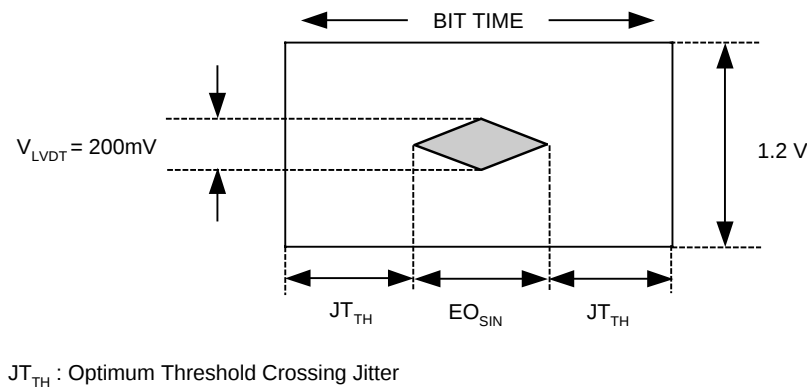
Figure 24. Receive Data Eye Diagram Template (Differential)
