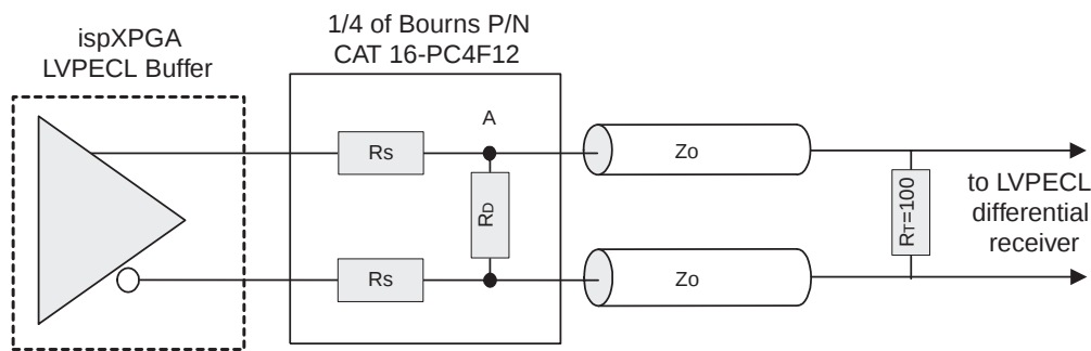
Figure 23. LVPECL Driver with Three Resistor Pack
