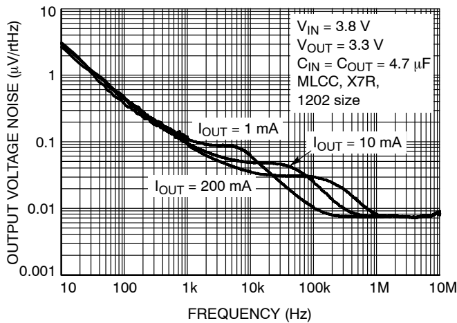
Figure 7. Output Voltage Noise Spectral Density for V_{\text{OUT}} = 3.3 \text{ V} , C_{\text{OUT}} = 4.7 \mu\text{F}
