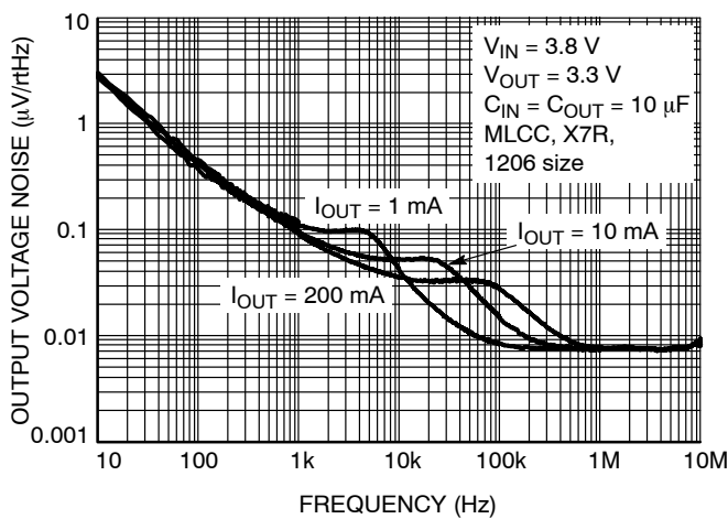
Figure 8. Output Voltage Noise Spectral Density for V_{\text{OUT}} = 3.3 \text{ V} , C_{\text{OUT}} = 10 \mu\text{F}
