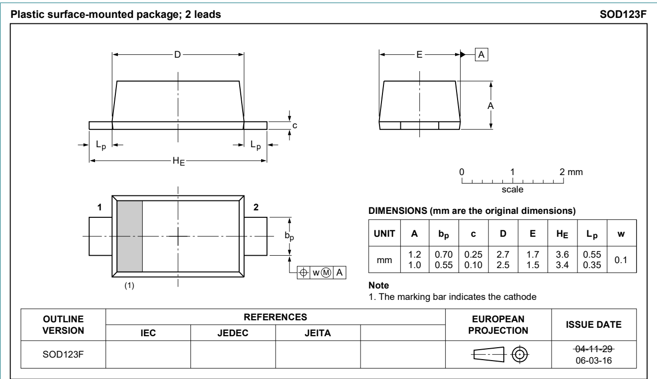
Fig. 5. Package outline SOD123F
