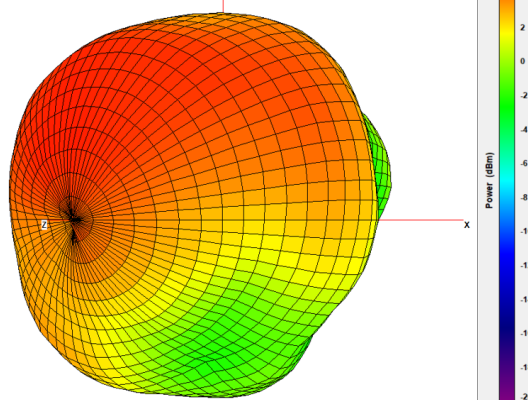
MIMO 2 – Free Space
