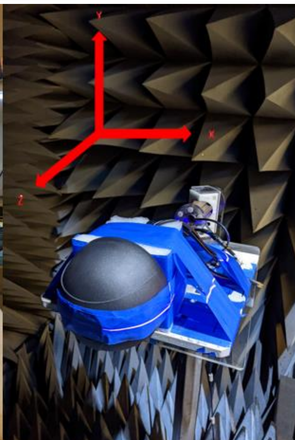
Chamber Test Set-up
