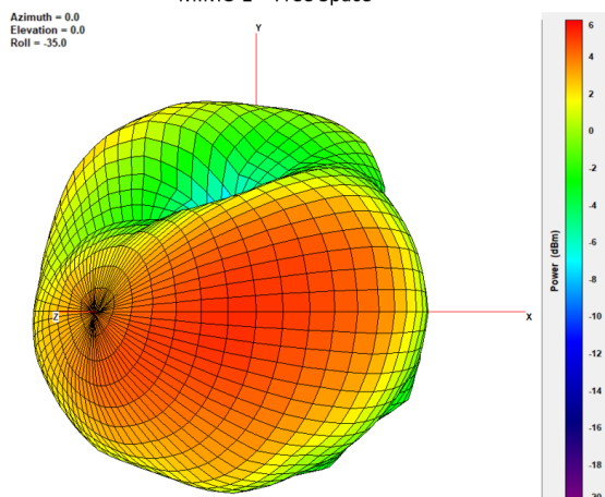
MIMO 1 – Free Space
