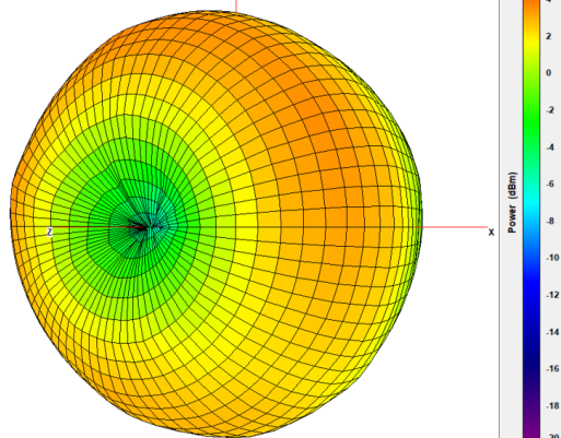
MIMO 1 – 30cmx30cm Ground Plane
