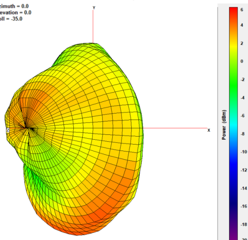
MIMO 1 – Free Space
