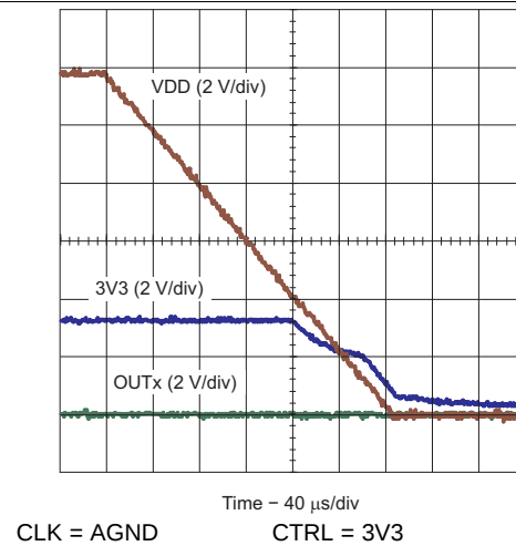
Figure 23. Shut-Down Behavior at V_{DD} = 12\text{ V}
