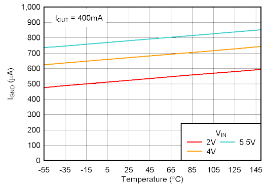
Figure 5-14. Ground Pin Current vs Temperature
