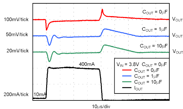
Figure 5-36. TPS73633 Load Transient Response
