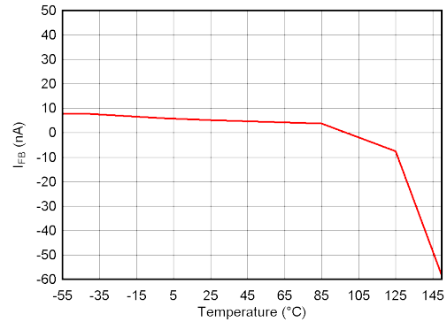
Figure 5-50. TPS73601 I_{FB} vs Temperature
