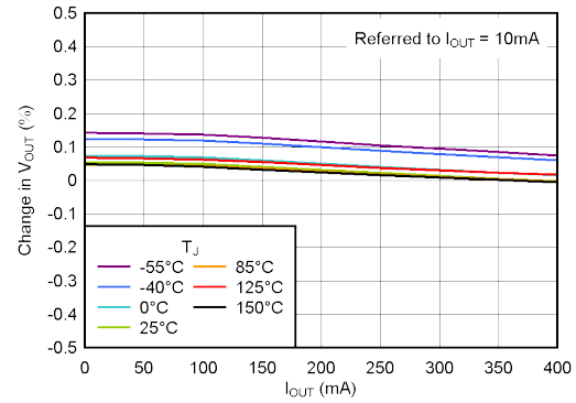
Figure 5-2. Load Regulation
