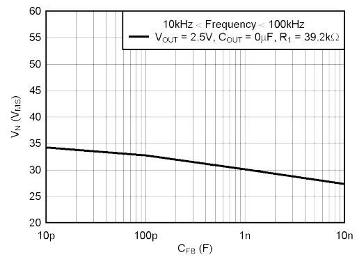
Figure 7-8. TPS73601 RMS Noise Voltage vs CFB
