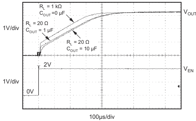
Figure 7-3. TPS73633 Turn-On Response
