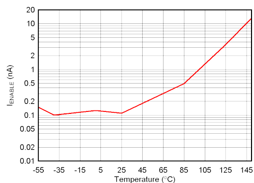
Figure 5-46. I_{ENABLE} vs Temperature
