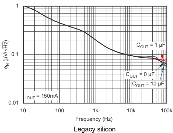
Figure 5-29. Noise Spectral Density C_{NR} = 0.01\text{ }\mu\text{F}
