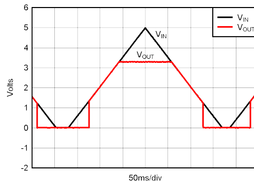
Figure 5-44. TPS73633 Power-Up, Power-Down
