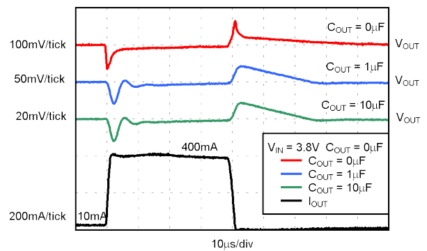
Figure 7-6. TPS73633 Load Transient Response
