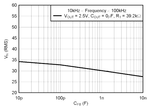
Figure 5-48. TPS73601 RMS Noise Voltage vs C_{FB}
