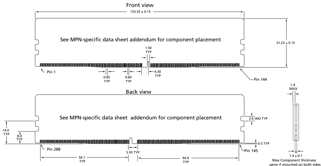
Figure 1: 288-Pin DDR4 UDIMM
