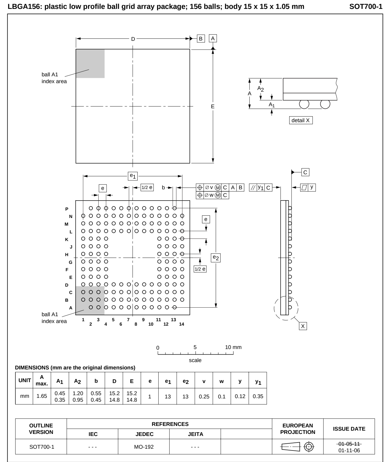
Fig 96. Package outline SOT700-1 (LBGA156)
