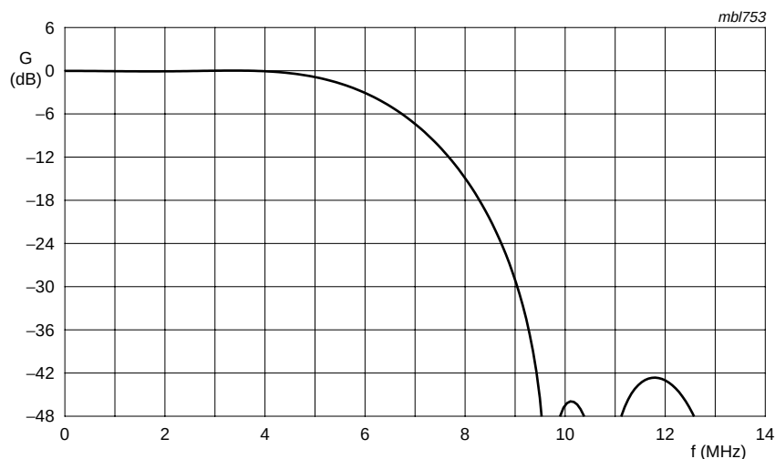
Fig 5. Decimation filter
