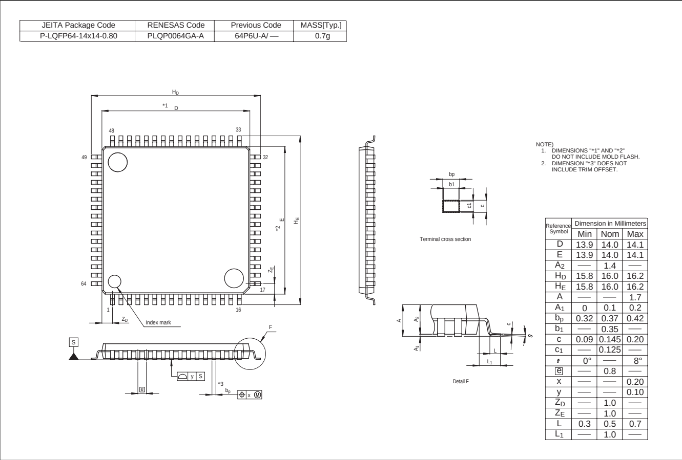
Figure A2.3 LQFP 64-pin 0.8mm pitch
