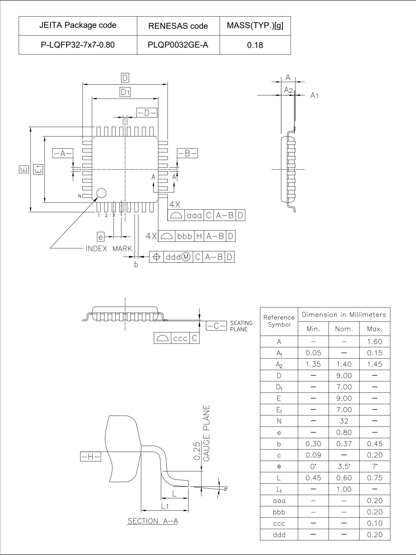
Figure A2.8 LQFP 32-pin (2)
