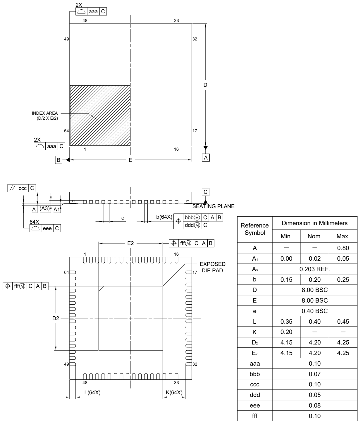
Figure A2.13 HWQFN 64-pin
