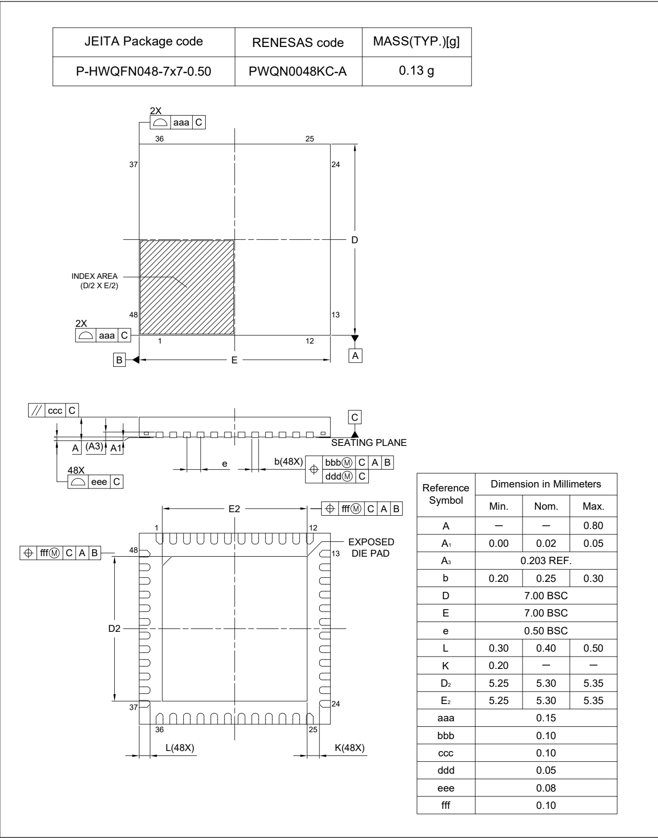
Figure A2.6 HWQFN 48-pin
