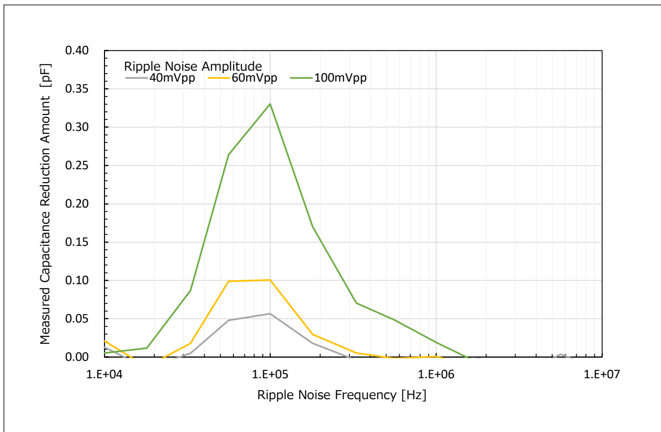
Figure 2.46 Measured capacitance reduction amount
