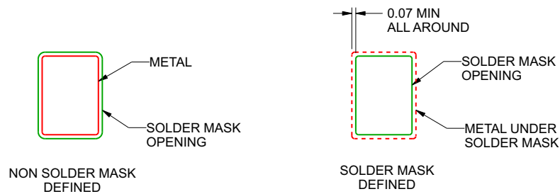
SOLDER MASK DETAILS NOT TO SCALE
