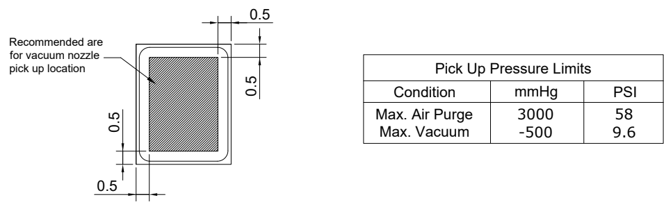
Figure 14. Pickup Tool Pick Location
