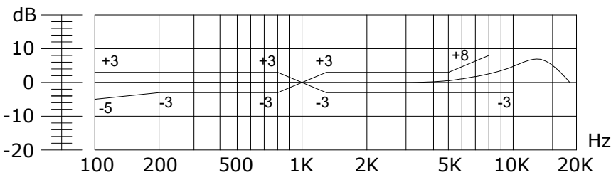
Figure 5. Frequency Response
