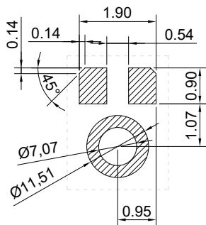
Figure 9. PCB solder pad layout for SMO06C-38
