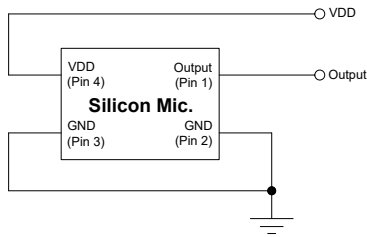
Figure 3. SMO06C-38 Interface Schematic Diagram
