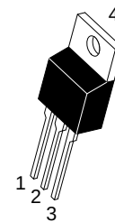
TO-220 CASE 221A-09 STYLE 1
