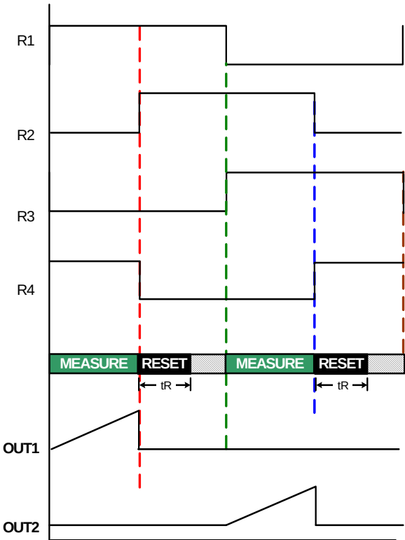
Figure 13. Full-Bridge Timing Example C
