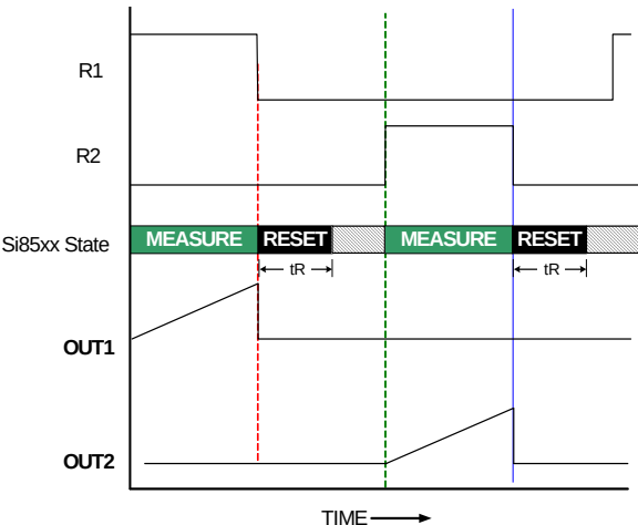
Figure 12. Full-Bridge Timing Example B
