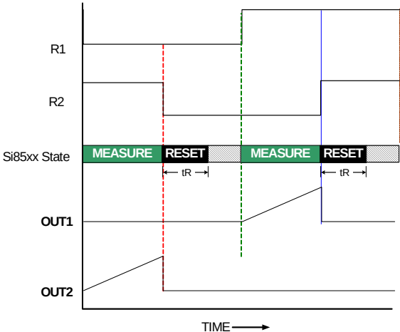
Figure 11. Two-Phase Buck Timing Example A
