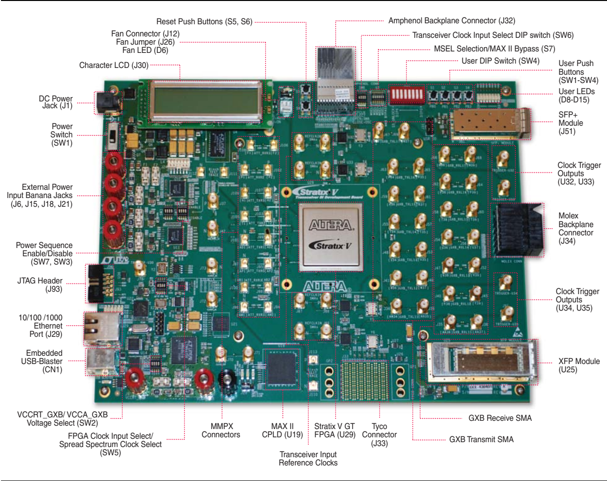
Figure 2-1. Overview of the Stratix V GT Transceiver Signal Integrity Development Board Features
