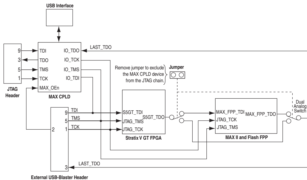
Figure 2-5. JTAG Header
