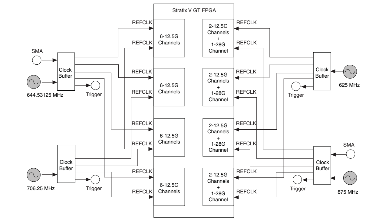
Figure 2–6. Transceiver Signal Integrity Development Kit Dedicated Transceiver Clocks
