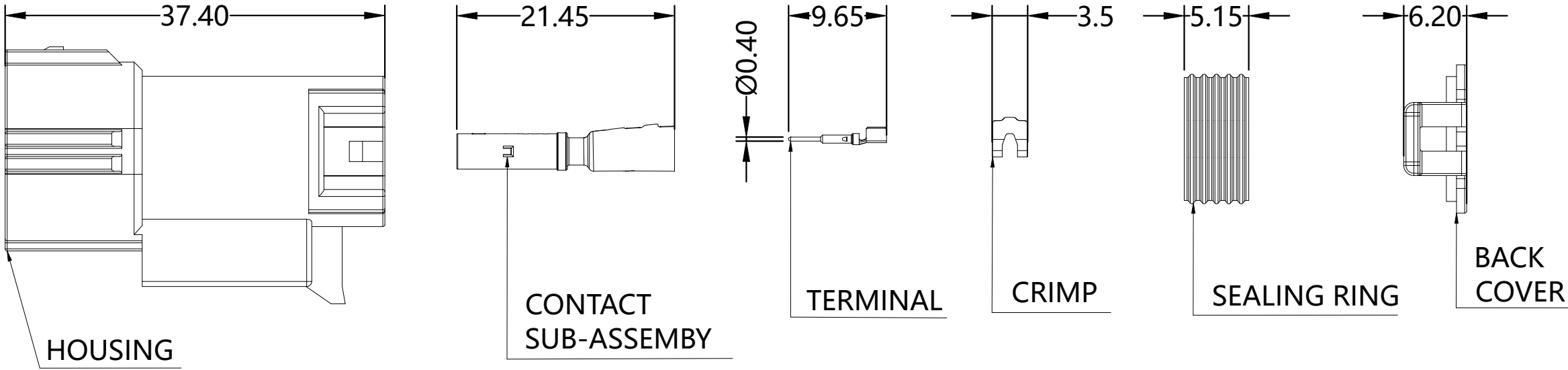
COMPONENTS TABLE: X-2545477-X FOR CABLE RTK031
