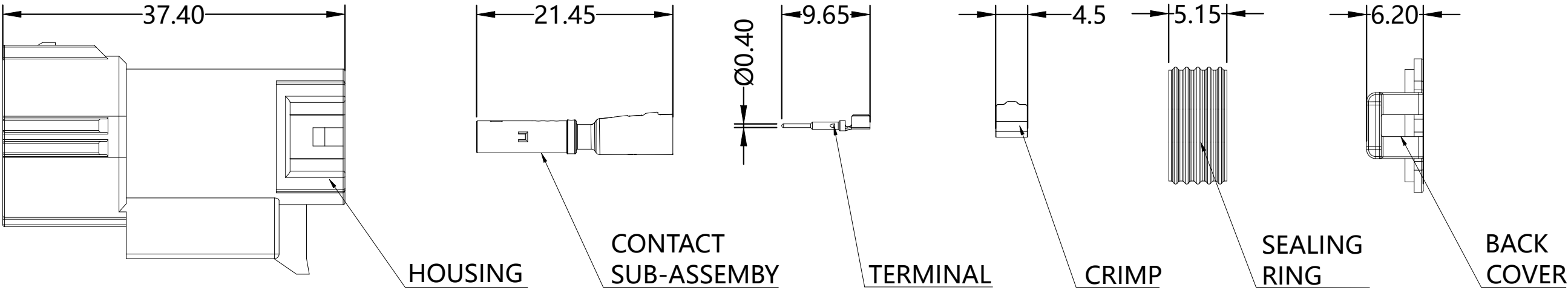
COMPONENTS TABLE: X-2545477-X FOR CABLE RG174
